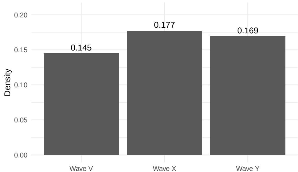
Network density across waves
